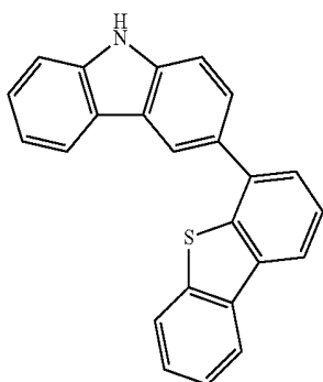
Step 1: Synthesis of 3-(Dibenzothiophen-4-yl)-9H-carbazole (abbreviation: DBTCz-II)
