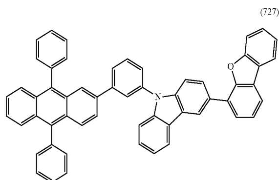
Step 1: Synthesis of 3-(Dibenzofuran-4-yl)-9H-carbazole (abbreviation: DBFCz-II)
